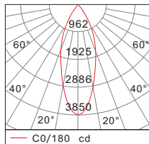
Photometric Diagram
