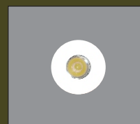
Binary Star
