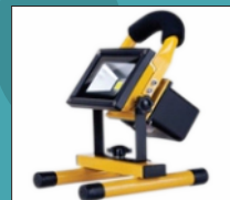
White Dwarf
