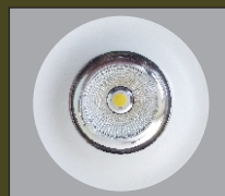
Comet Star
